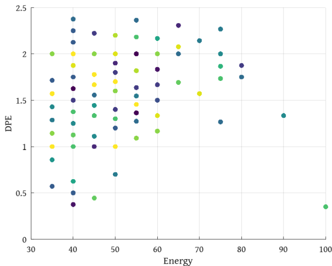
Figure 7.3: PPE vs energy for charged attacks
